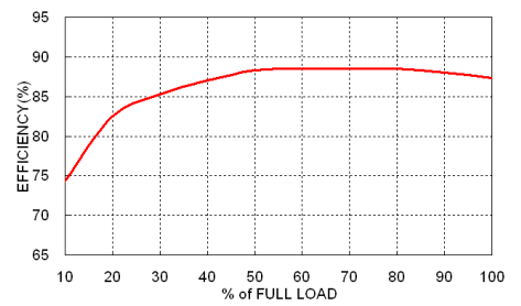
DFEC40-48S05 Efficiency vs. Output Load
