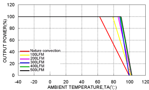
FED40-48S05W Derating Curve
