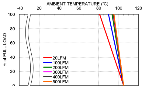
LCD10-48S05 Derating Curve
